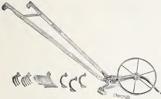
No. 16 Single Wheel Hoe—Here is a very complete, light running cultivating tool suitable for either the home or market garden .....$9.00
